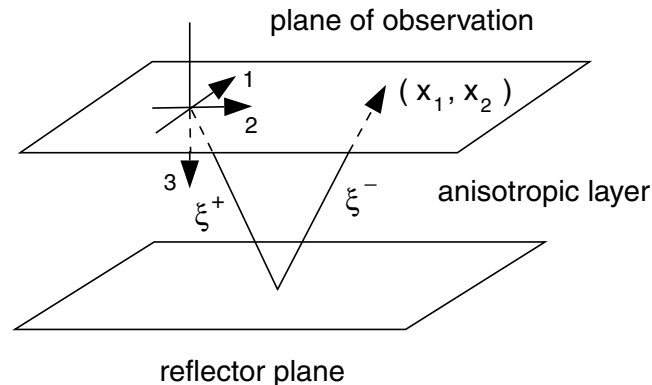
Figure 1. A seismic ray is reflected at a plane interface which is parallel to the plane of observation.
